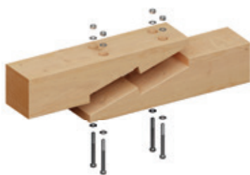
Haaklasverbinding
